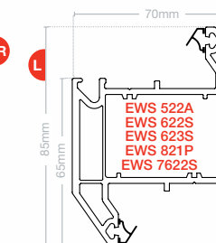
Intermediate transom Z EWS 7023
