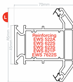
Intermediate transom T EWS 7022
