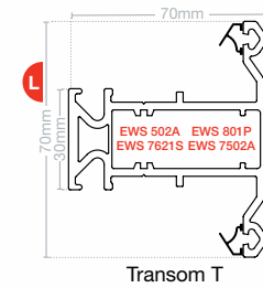
Transom T EWS 7002
